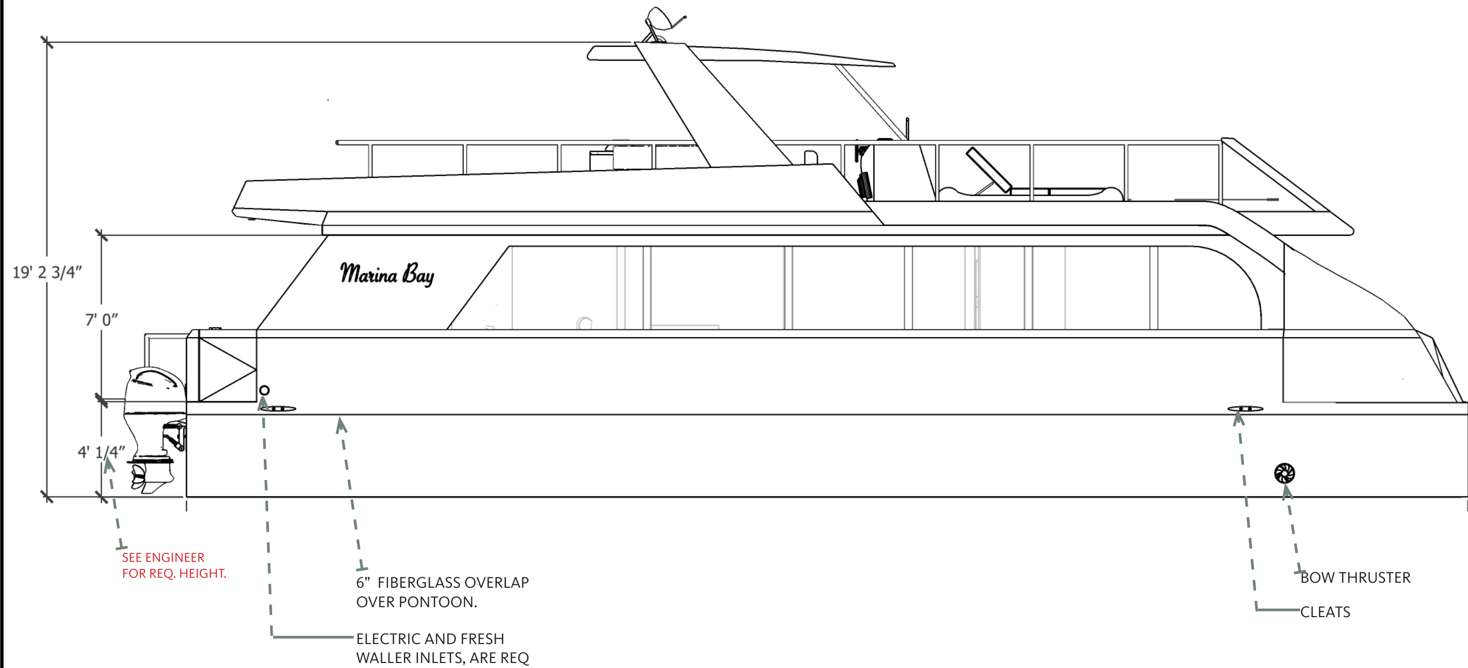
EXTERIOR SIDE ELEVATION
