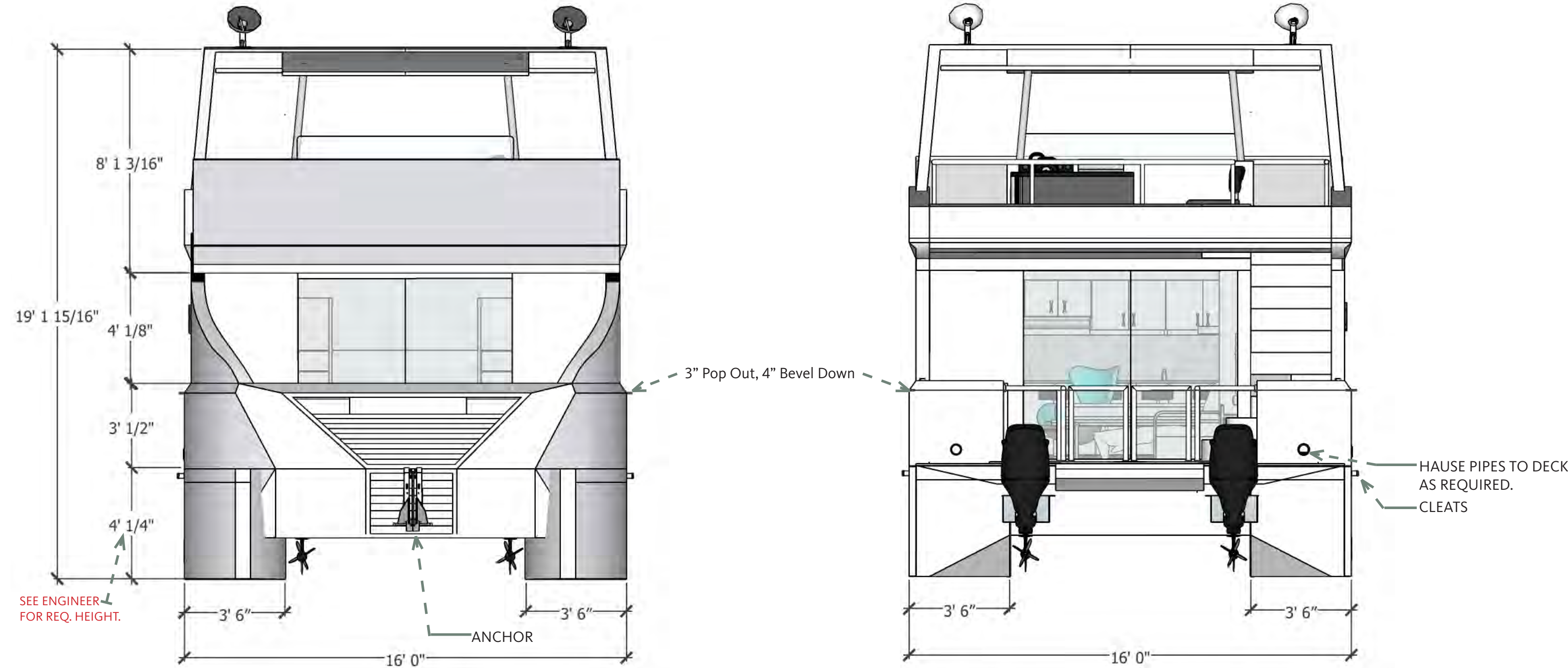
EXTERIOR ELEVATIONS
