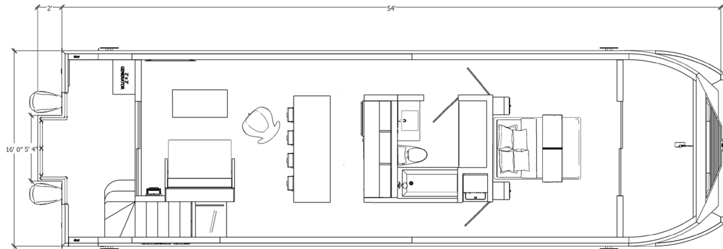
MAIN FLOOR PLAN
