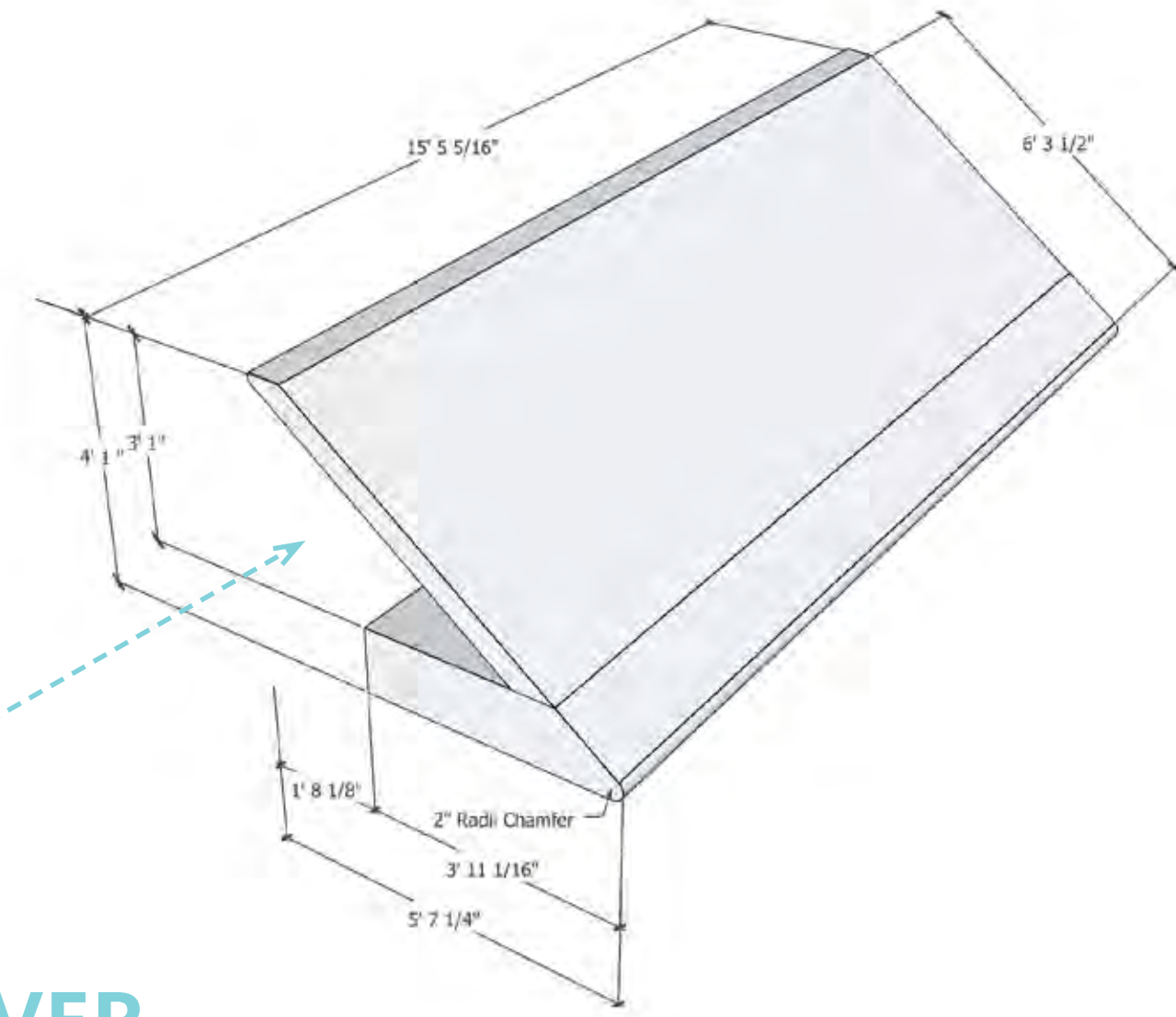
BOW DETAILS
